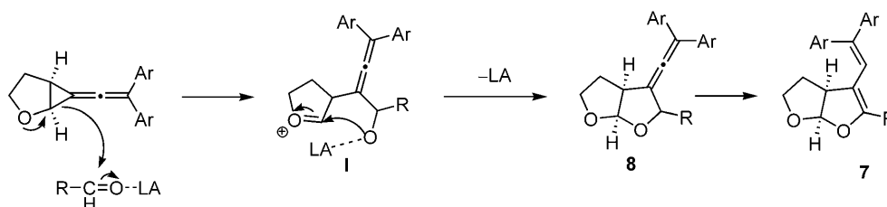
Scheme 3. Proposed mechanism.
