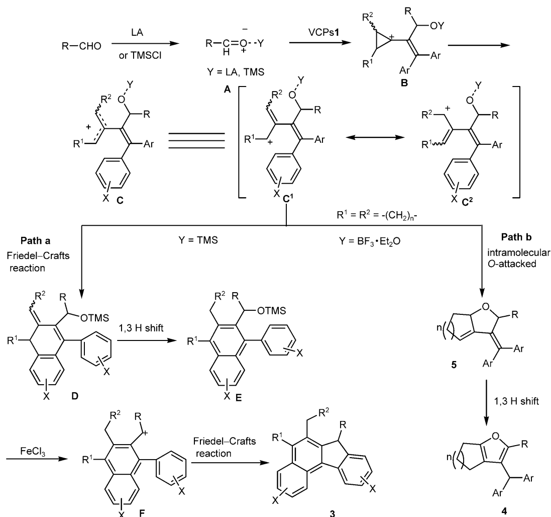
Scheme 2. Proposed mechanism for the synthesis of benzo[ c ]fluorene derivatives 3 and furan derivatives 4 .
