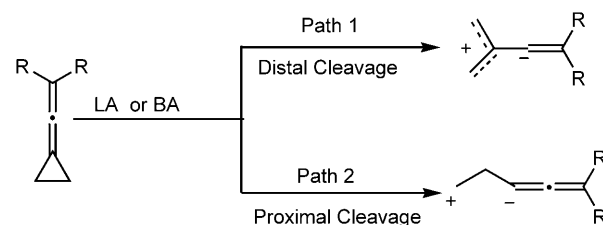
Figure 1. Lewis acid- or Brønsted acid-mediated ring opening reaction models for VCPs.
